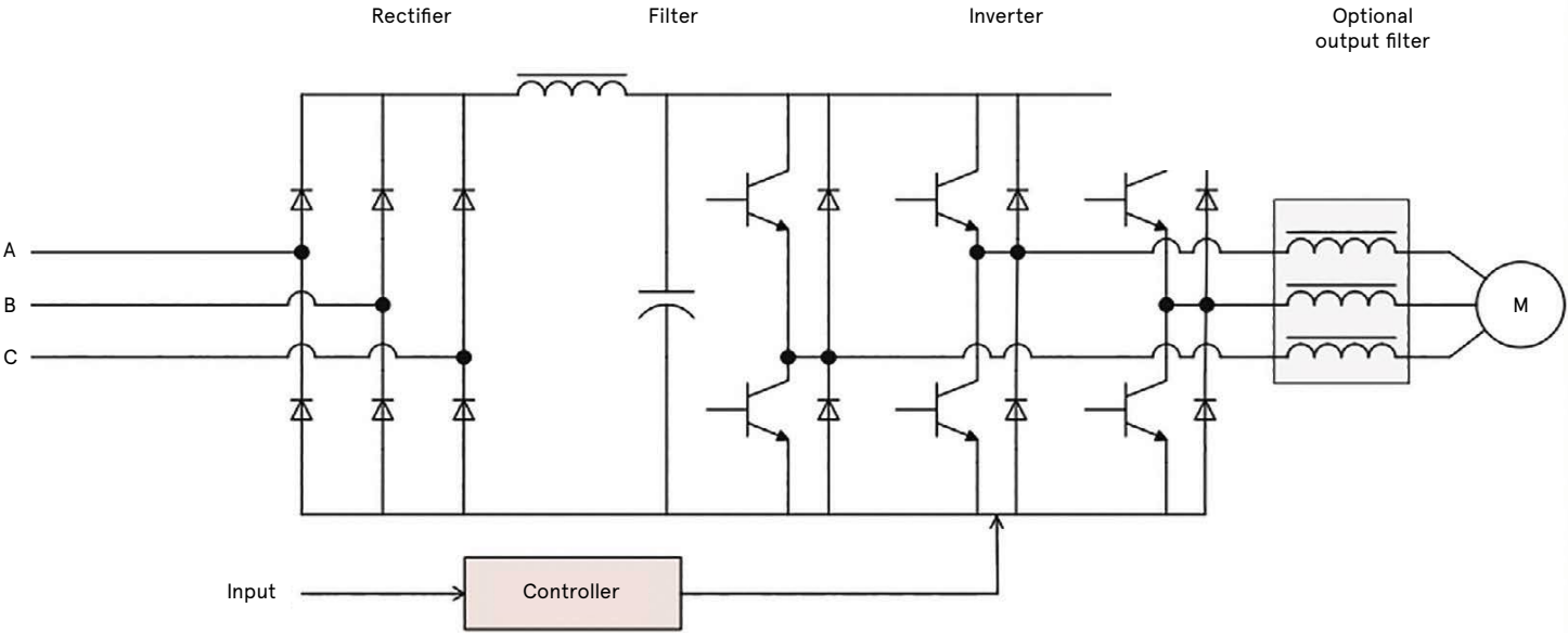
Figure 6: Active front end
